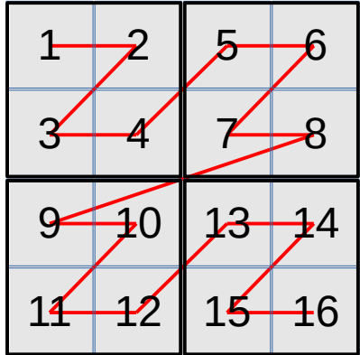
Z-order curve
